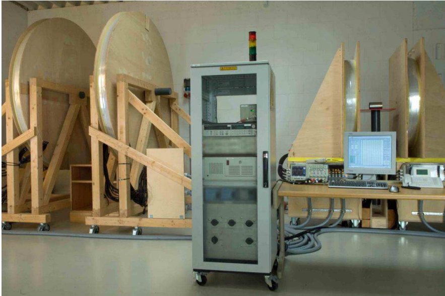
Fig. 2: Helmholtz coil systems to measure shielding factors and to simulate electro-magnetic interferences.
