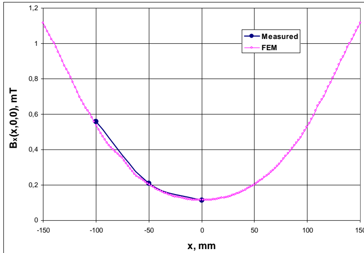
Fig. 3: Measured and simulated axial magnetic field B_x(x) along the symmetry axis of an open, circular MUMETALL® cylinder, aligned coaxially in the centre ( x = 0 ) of a Helmholtz coil system. The lines between the dots are guides for the eye only.
