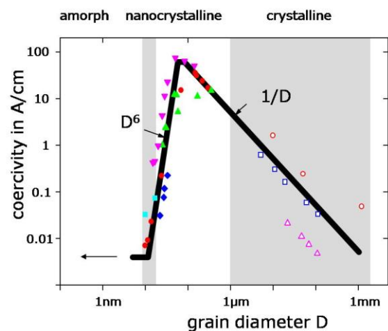
Fig 2 The famous D^6 law from Dr. Herzer: making things smaller will sometimes surprise
