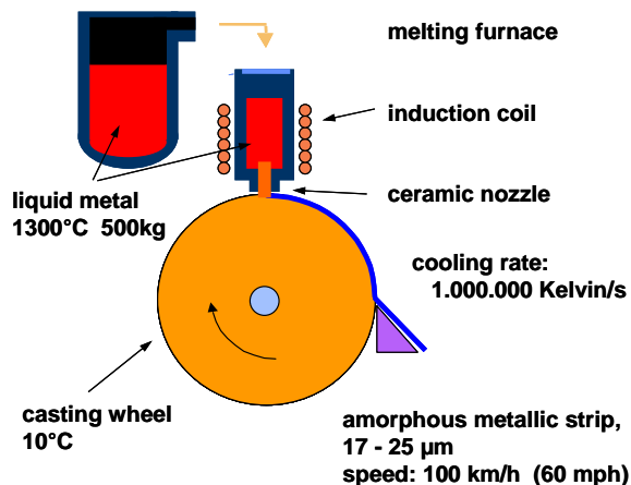
Fig 3 Rapid Solidification Technology
