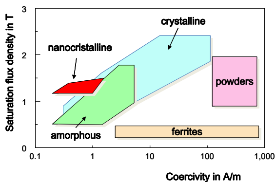
Fig 1 Overview of soft magnetic alloys: not complete but hopefully enough to demonstrate
