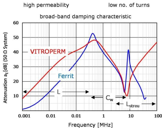
Fig 7 Damping behavior of nanocrystalline common mode chokes - small size, broadband, almost no degradation at high temperatures
