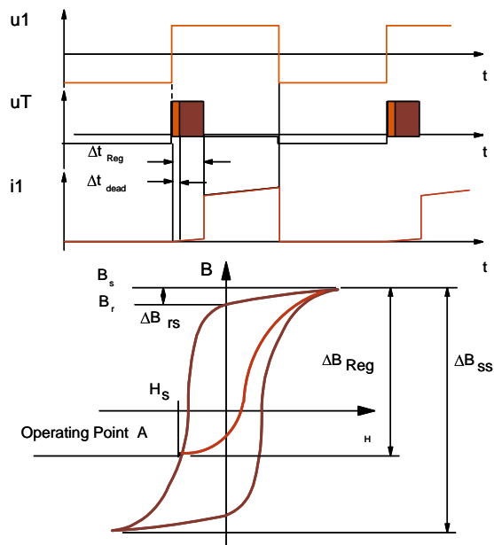
Fig 6 Basic principle of a MagAmp: During the magnetization from operating point A to saturation, the voltage drops across the MagAmp choke. This part of the wave is removed from the full square wave. Since the operating point can be manipulated (via the regulation circuit), the part which is taken away can be regulated and therefore also the output voltage.
