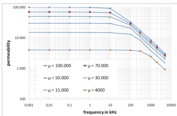
Fig. 5 Permeability versus frequency of nanocrystalline cores with different permeability levels
