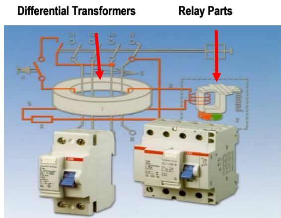
Fig 9 Basic GFCI design (European version)
