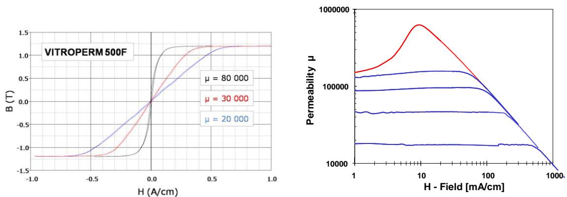
Fig. 4 Static hysteresis loops and permeability versus field strength of nanocrystalline cores with different permeability levels. The red curve on the right is the characteristic w/o magnetic field annealing (unpublished results from Dr. Petzold, Vacuumschmelze GmbH & Co. KG)
